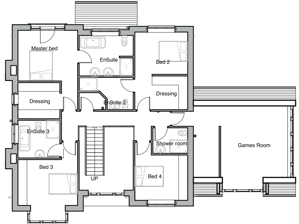
First floor
